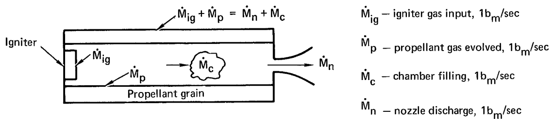
Figure 14.—Mass balance system.
