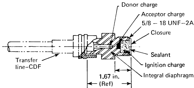
Figure 6.—Through-bulkhead initiator.
