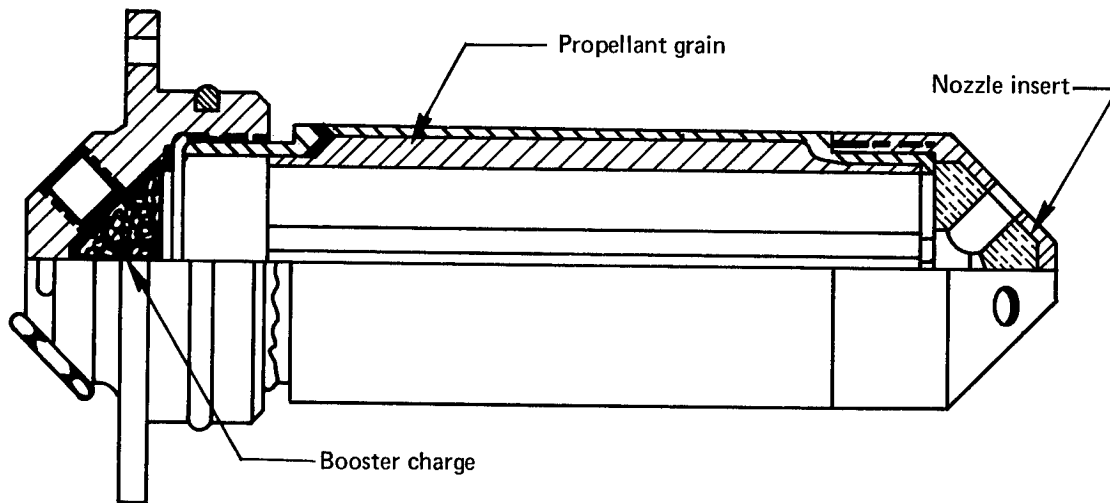
Figure 7.—Pyrogen igniter.
