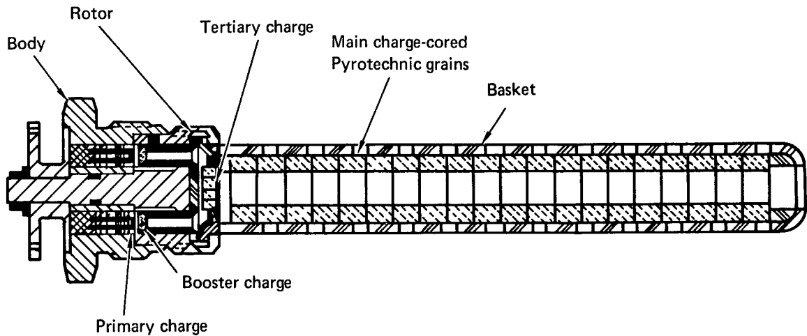
Figure 8.—Pyrodyne igniter.
